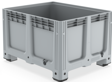
100x120x76 (h)cm
