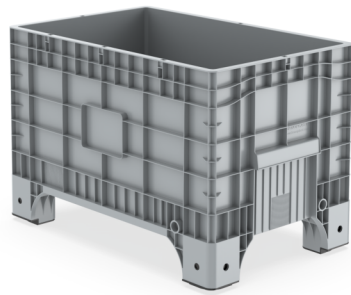
65x100x67 (h)cm
