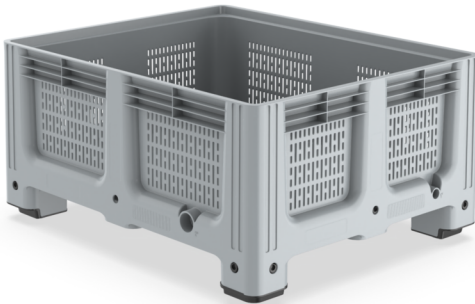
100x120x58 (h)cm
